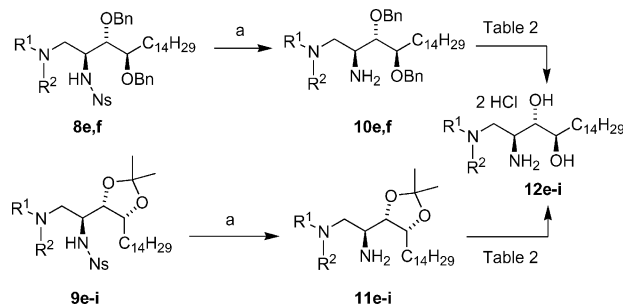
Scheme 3. Sequential deprotection of 1,2-diaminophytosphingosines. Reaction conditions: (a) \text{PhSH} (4 equiv./mol)/ \text{Cs}_2\text{CO}_3 (3 equiv./mol), \text{CH}_3\text{CN} , room temp., 20 h. For compound identification and yields, see Table 2.
