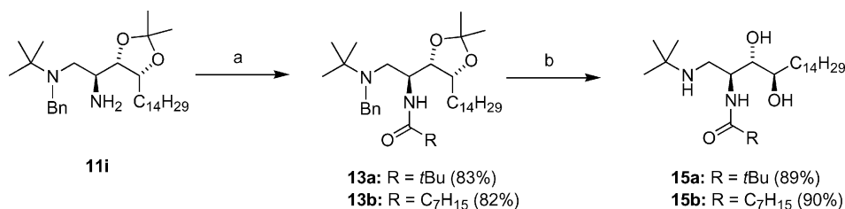
Scheme 4. Acylation of diamines 11 and simultaneous N - and O -deprotection. Reaction conditions: (a) RCOCl, THF, Et 3 N; b) H 2 , 5% Pd/C, HCl, MeOH.
