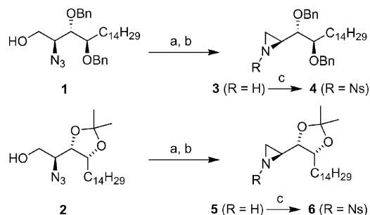
Scheme 1. Reagents and conditions: (a) \text{MsCl} , THF, \text{Et}_3\text{N} ; (b) \text{Ph}_3\text{P} , THF, \text{H}_2\text{O} ; (c) \text{ClSO}_2\text{R} , THF, \text{Et}_3\text{N} .
