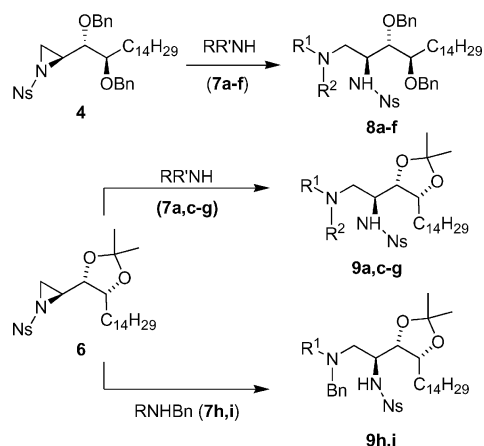
Scheme 2. Ring-opening of nosylaziridines with amines. Reaction conditions: amine (2 equiv./mol), \text{CH}_3\text{CN} , reflux, 3 h or room temp. 24 h. For compound identification and yields, see Table 1.
